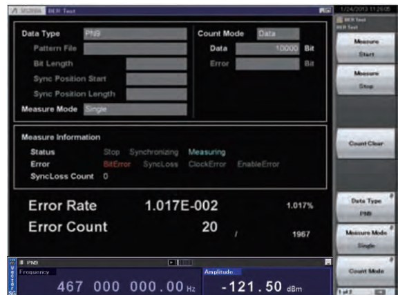
BER Measurement Function (top) and Vector Signal Generator (bottom) Measurement Examples
